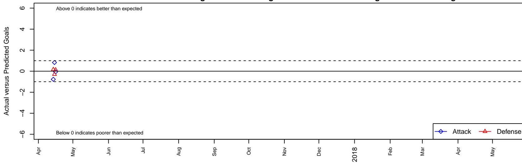
Surrey United B99 Dots are actual minus expected GF (blue circles) and GA (red triangles). Blue line is smoothed change in attack strength. Red is smoothed change in defense strength.
